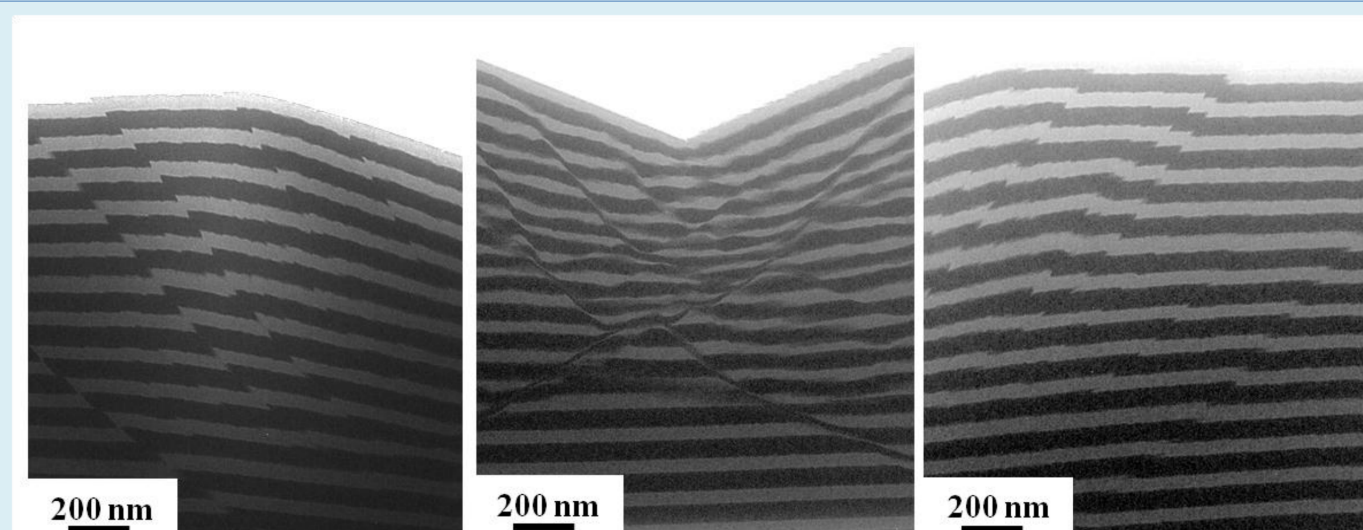
The enlarged views of the shear bands indented to 1000 nm.
