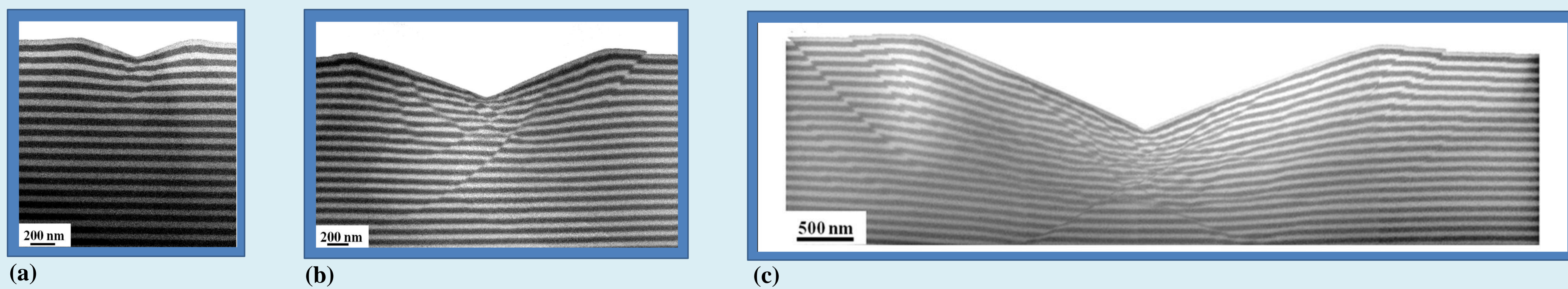
Full view of shear bands patterns beneath nanoindentation indented to (a) 200nm, (b) 500 nm and (c) 1000 nm.
