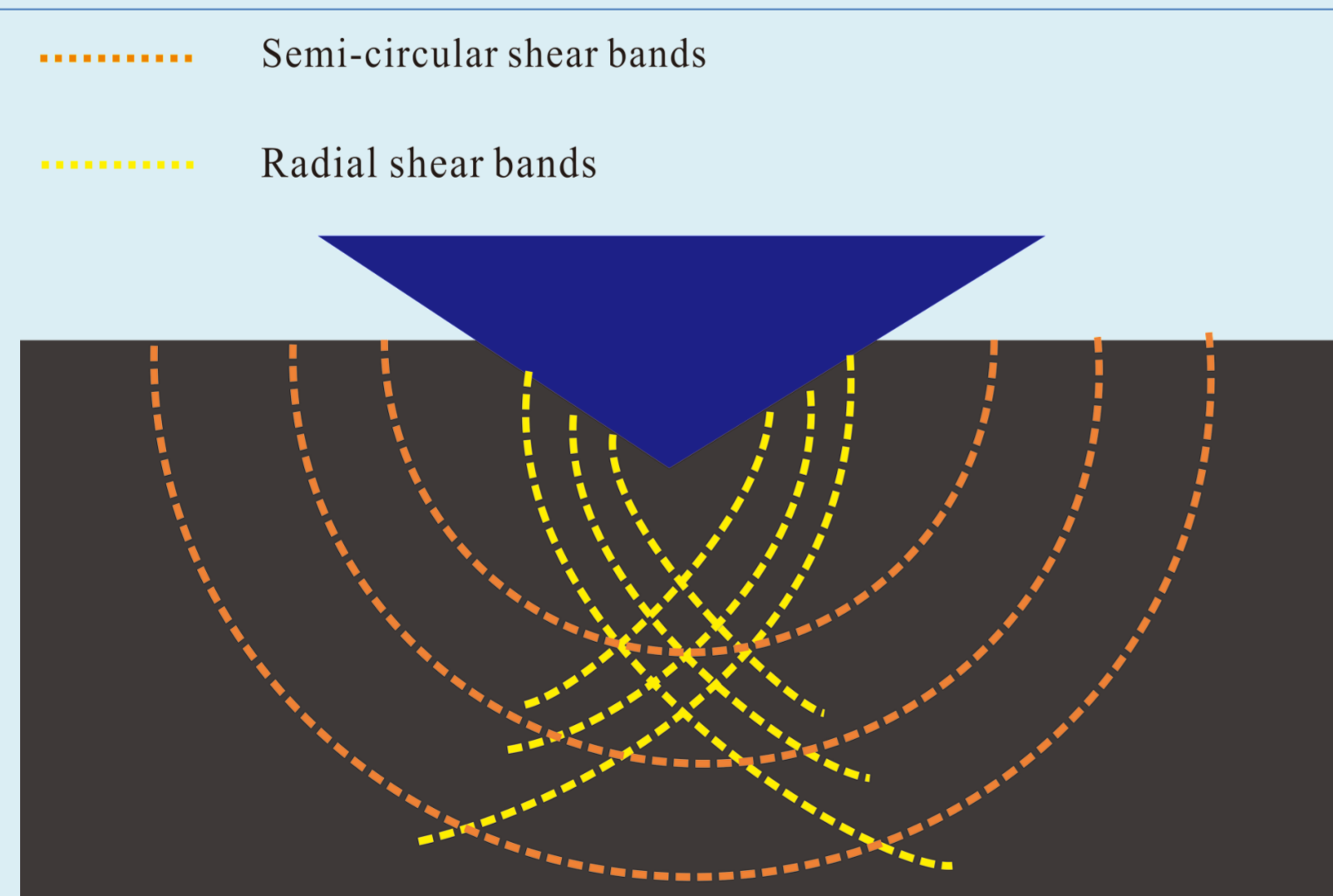
Expanding cavity model
